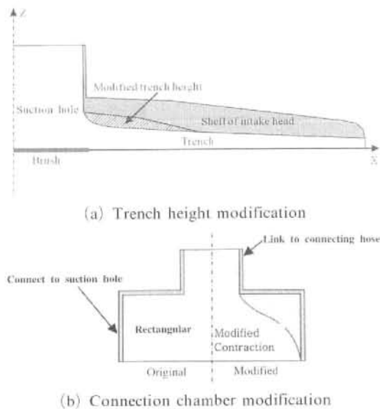
Fig. 3 Schematic diagram of trench height modification and modified connection chamber
