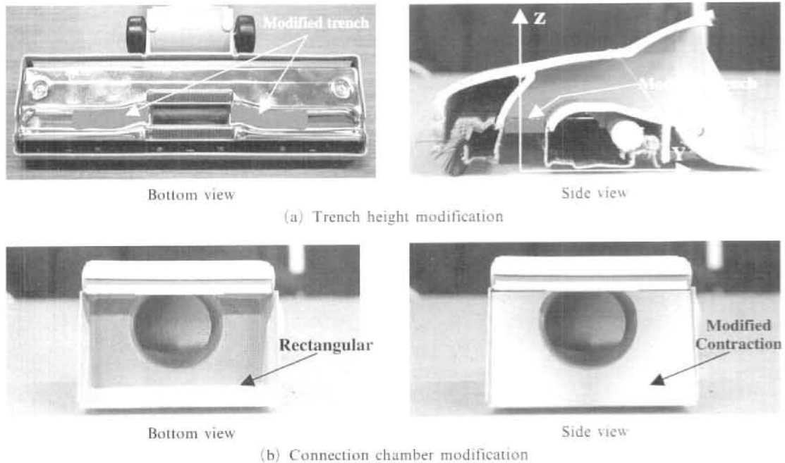
Fig. 2 Photographs of airflow paths of modified intake heads
