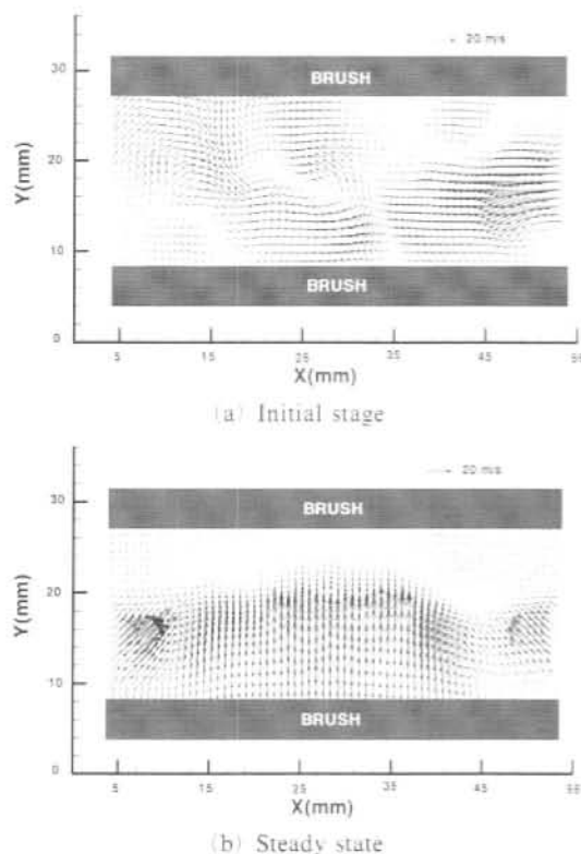
Fig. 11 Instantaneous velocity field for intake head modified in both connection chamber and trench height
